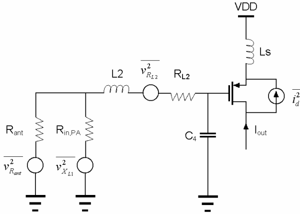
Fig. 3. Noise model of the LNA
